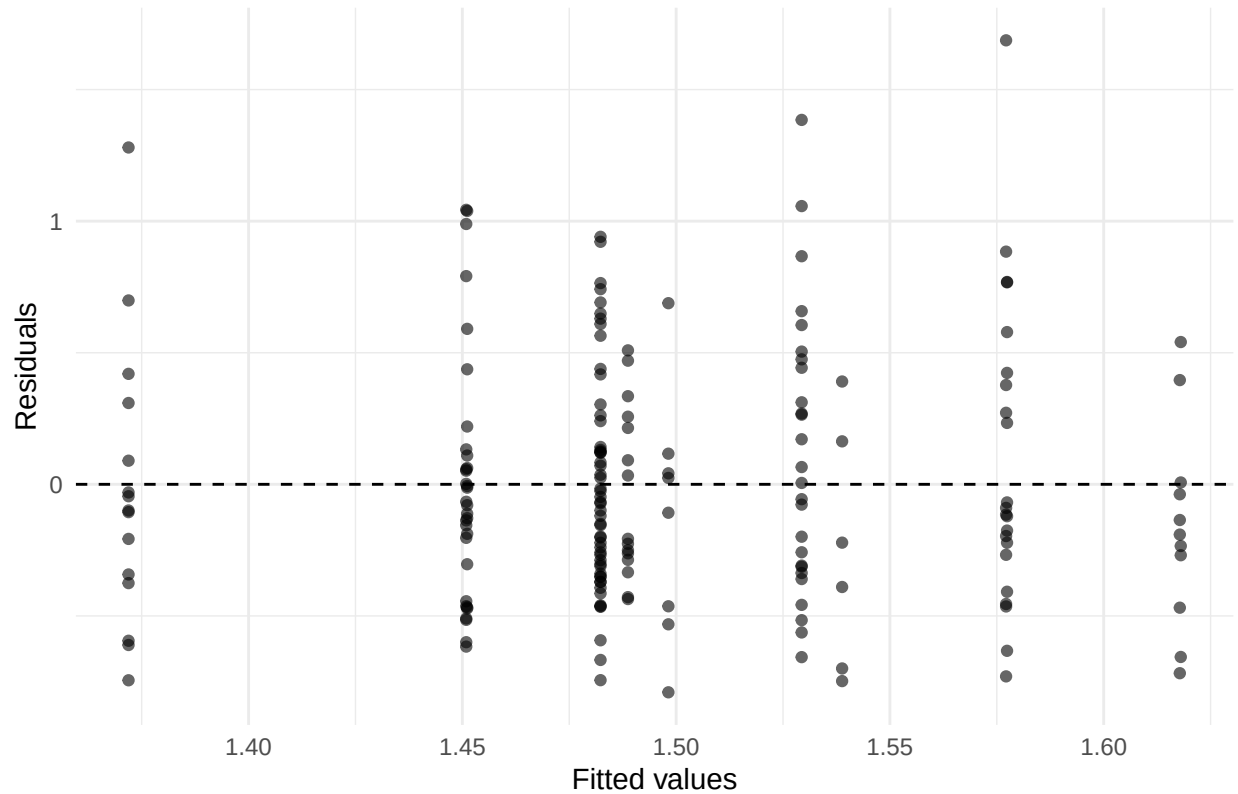
Residuals vs Fitted – Autoregressive
